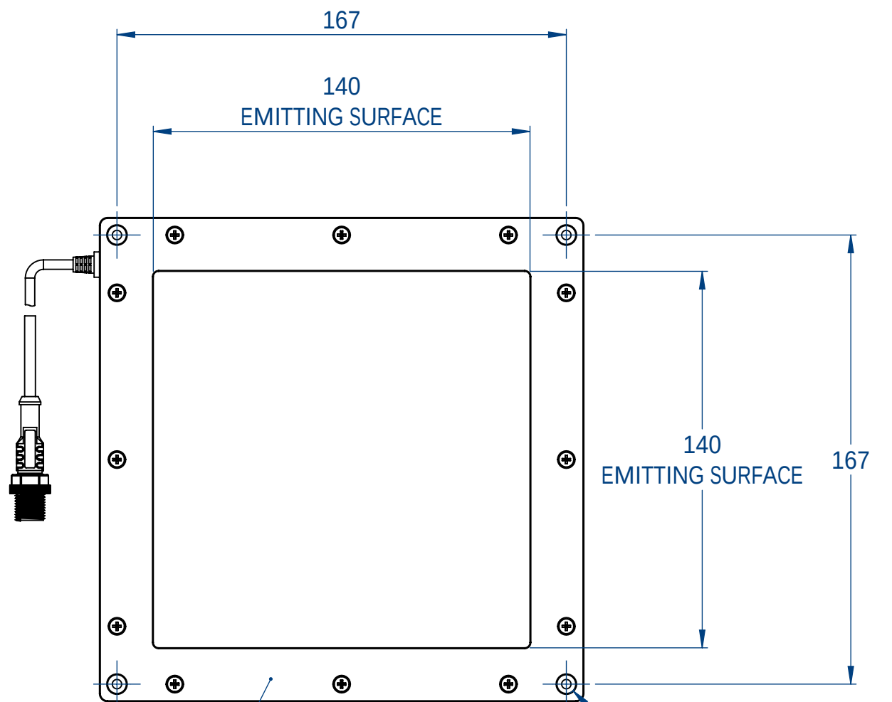
UPPER SIDE
